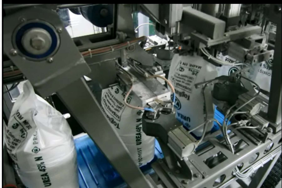
Axial mechanism
